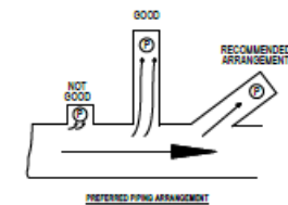
PREFERRED PIPING ARRANGEMENT
