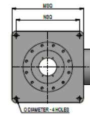
DISCHARGE BASE DIMENSIONS
