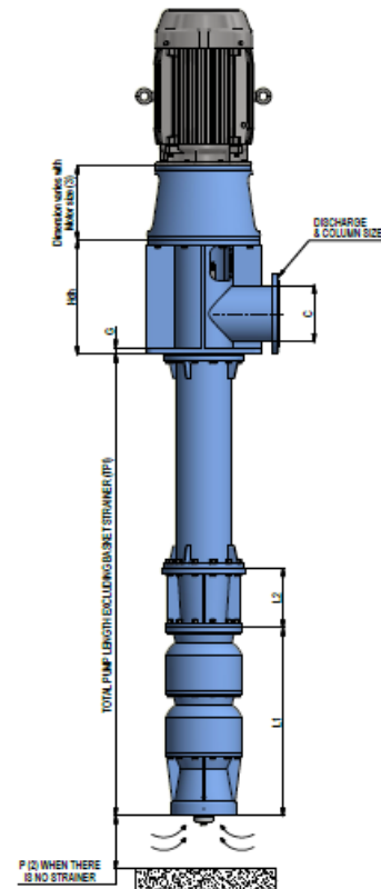
DISCHARGE BASE DIMENSIONS
